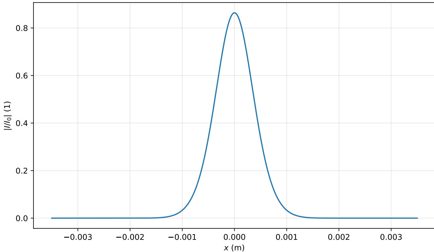
Intensity profile I(x, y = 0, z = 1.274m)/I_0 , P_{in}=0.3P_{cr} , artificial time
